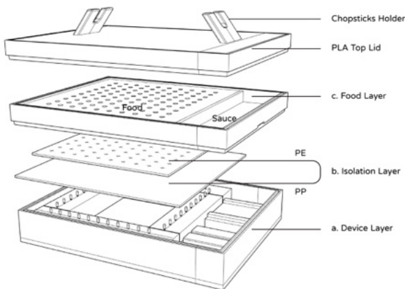
Figure 6: Mechanical Design
